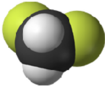
R32 molecule
